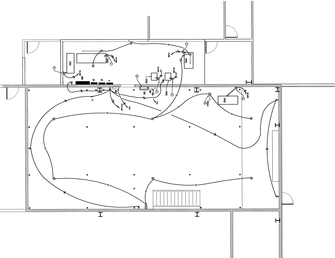
MEZZANINE POWER & LOW VOLTAGE FLOOR PLAN SCALE: 1/4" = 1'-0"
